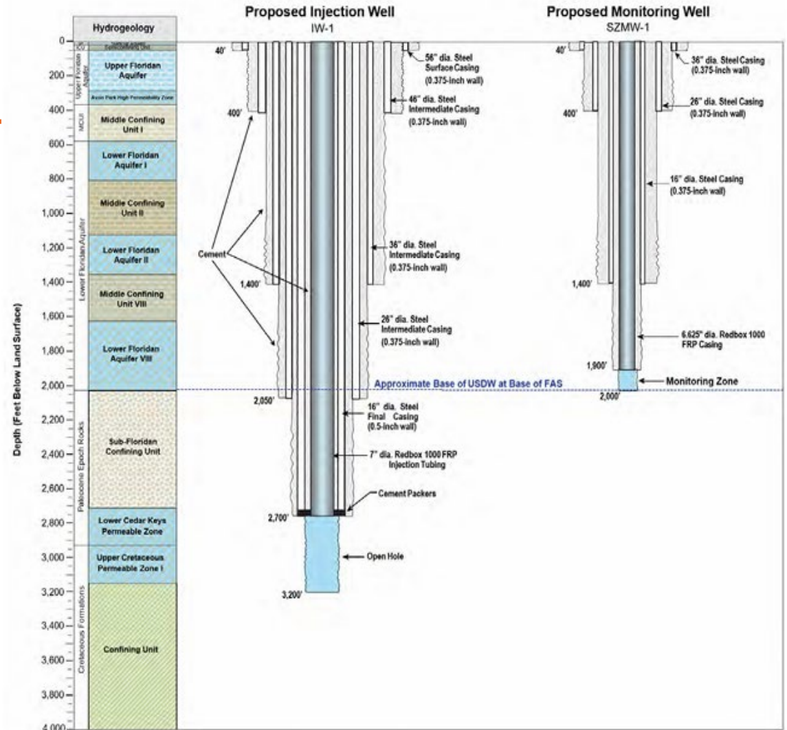
Figure 2-2 Wells IW-1 and SZMW-1 Design Schematic
