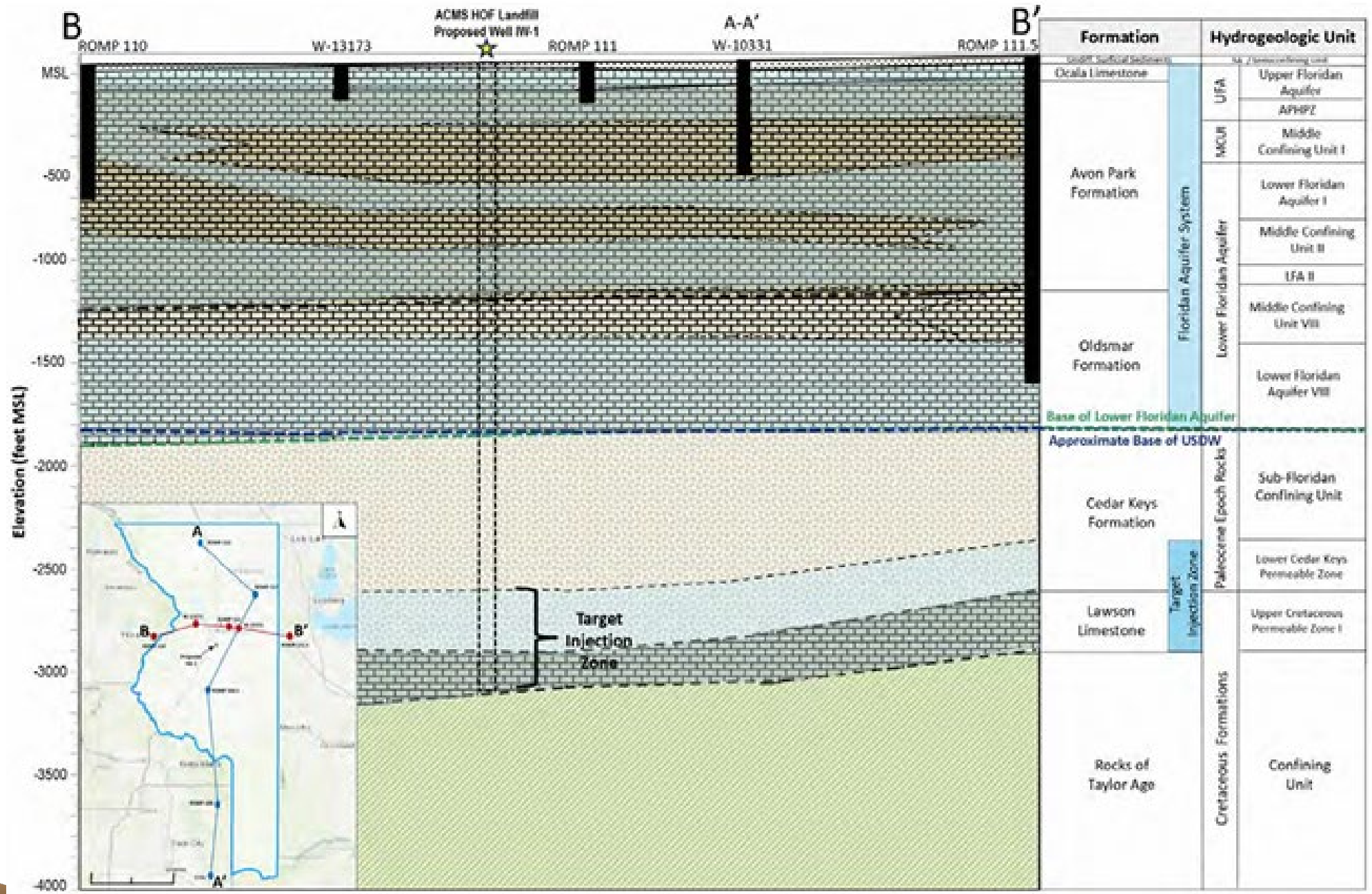
Figure 3-9 East West Cross Section B-B'
