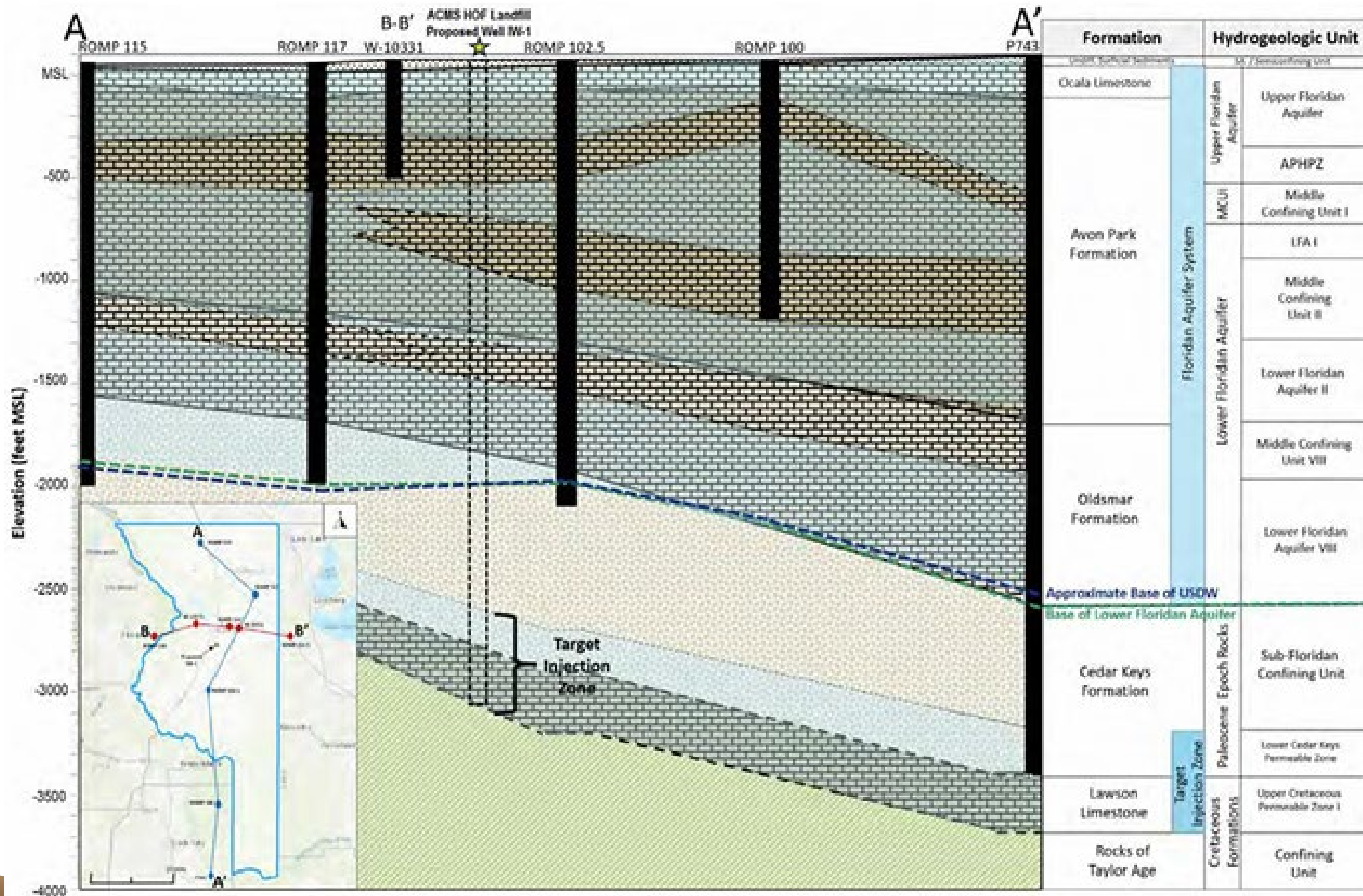
Figure 3-8 North South Cross Section A-A'
